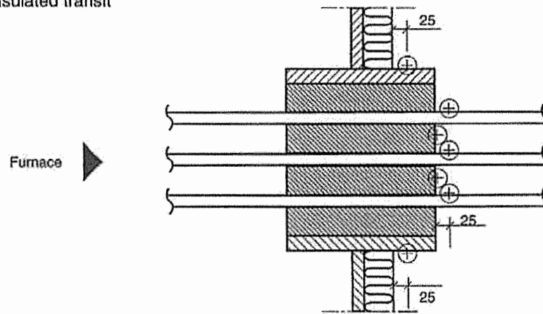
Uninsulated transit
