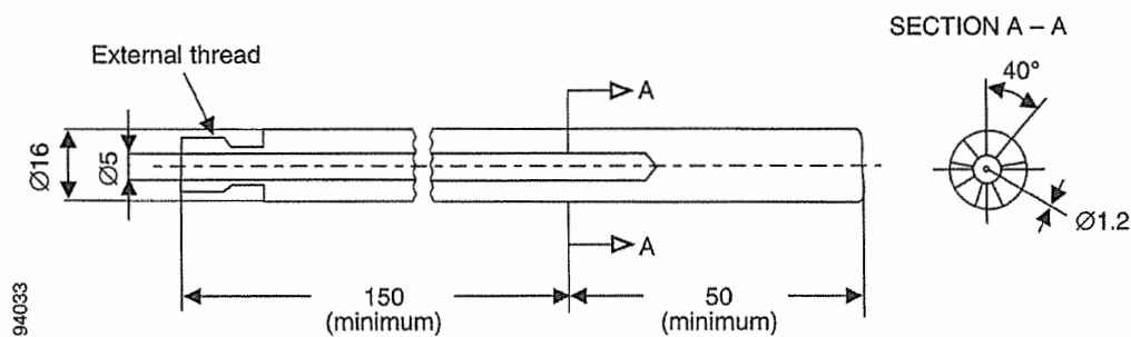
Figure 5 – Pressure-sensing heads
