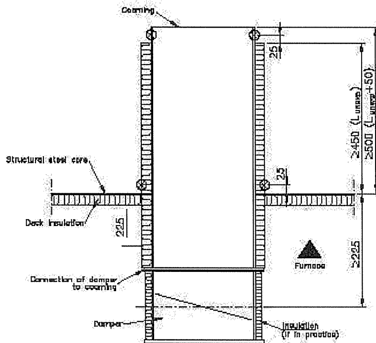
Deck specimen
