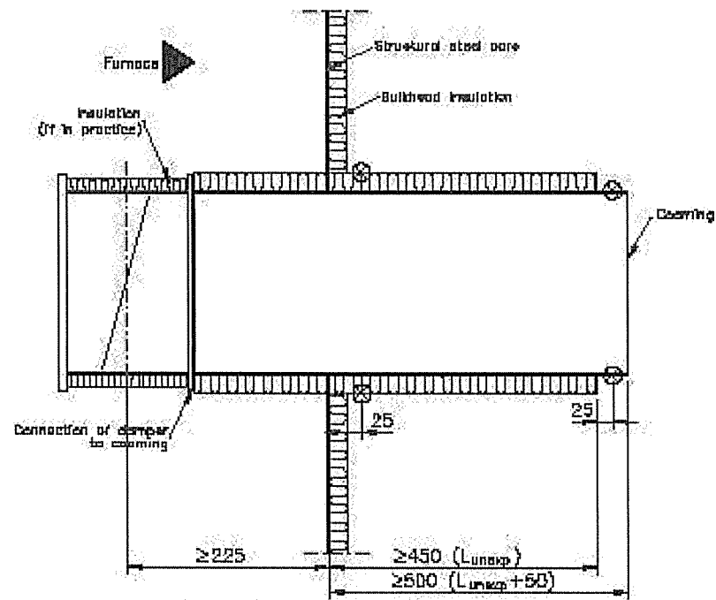
Bulkhead specimen
